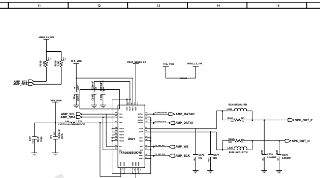
Audio amp
